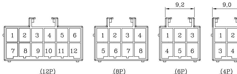
PIN ASSIGNMENT (Front View)
