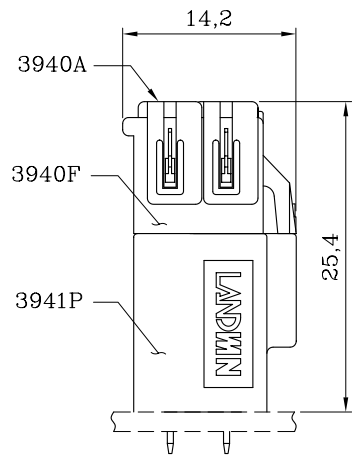
ASSEMBLY LAYOUT
