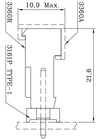
ASSEMBLY VIEW
