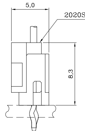
ASSEMBLY LAYOUT
