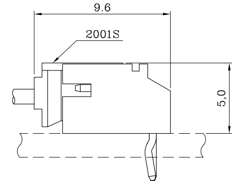
ASSEMBLY LAYOUT
